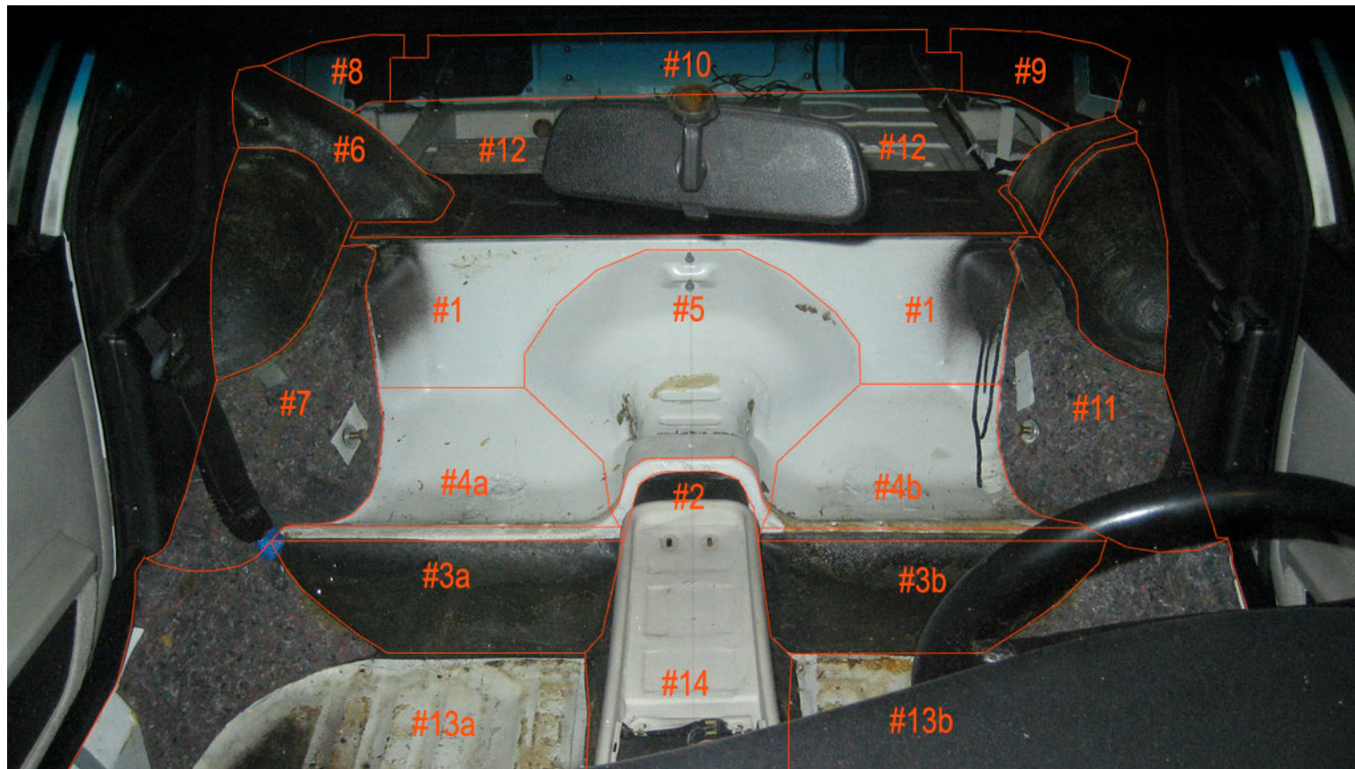
Layout - (Rear Seat Delete Kit)
